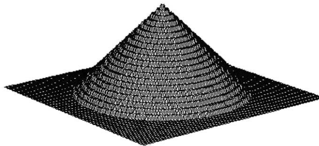
FIGURE 2. Letting \varepsilon \rightarrow 0 .
